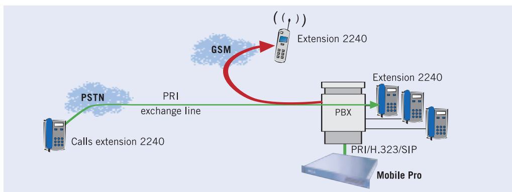
Without ECOTEL® VTM pro: The mobile phone and the fixed line phone both ring. If the employee takes the call on the mobile phone, high connection charges are incurred unnecessarily
