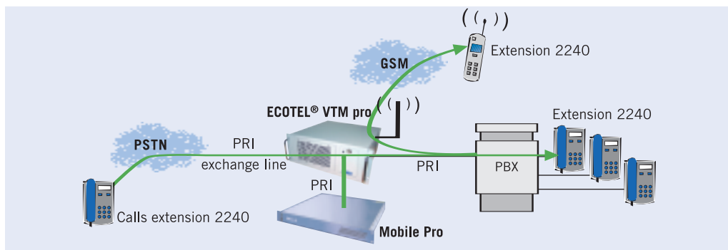
With ECOTEL® VTM pro: Connection charges for GSM networks are significantly decreased with mobile-to-mobile call routing
