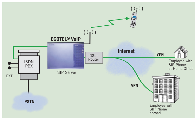
Connection via VPN
