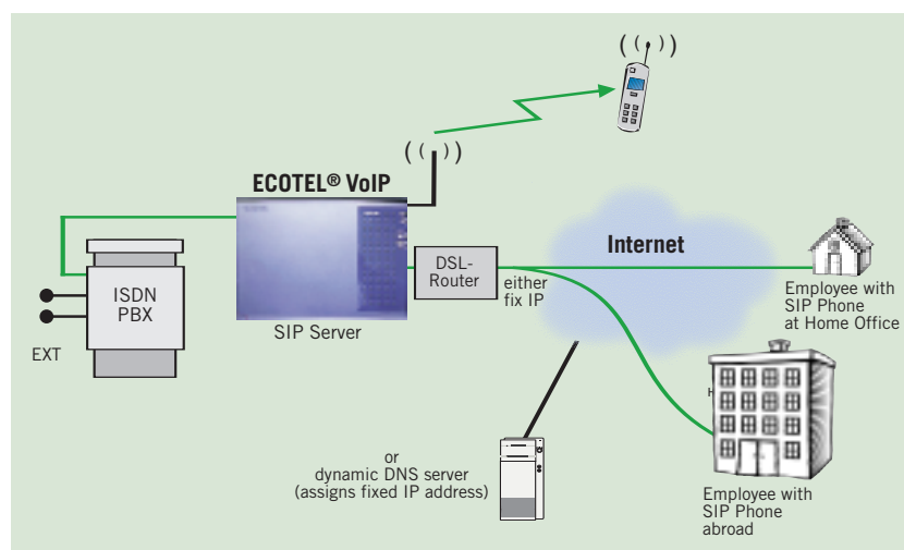
Connection without VPN
